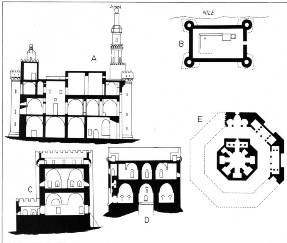
(A) Section through the central keep and mosque of Qayt-bay's fortress overlooking Alexandria harbour, 1479. (B) Plan of Qayt-bay's small fort overlooking the Nile north of Rashid, 1479 (after De Cosson). (C) Restored section through the 'Rivermouth Tower', Tripoli, Lebanon, c.1475, with additional bastion on left dating from the 17th-18th cents. (after Sauvaget). (D) Section through the 'Lions Tower', Tripoli, Lebanon, c.1475 (after Sauvaget). (E) Plan of the Qal'at al Tina, Sinai, probably built for Sultan al Ghuri in the early 16th cent. (after Tamari).
